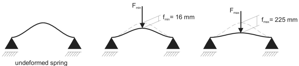
Figure 1. Spring life dynamic testing
